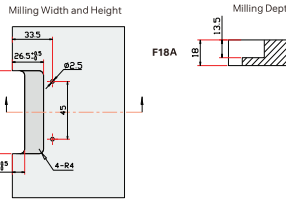
Milling Width and Height
