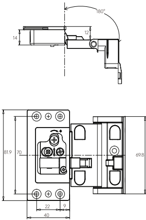
Milling and boring on side panel Full overlay Note: Side panel min. thickness 18mm when full overlay
